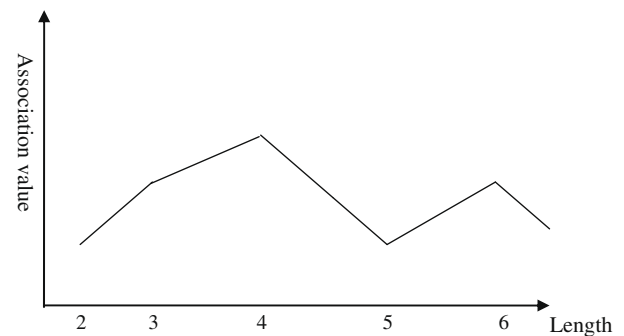
Fig. 4. CO assumes association value of a substantival MWE is monotonically increasing to its length while LocalMaxs use the local maxima as correct length. If LocalMaxs method is employed, then both 4-length and 6-length candidates will be assigned as MWEs. However, for CO, only 4-length will be assigned as a substantival MWE.
