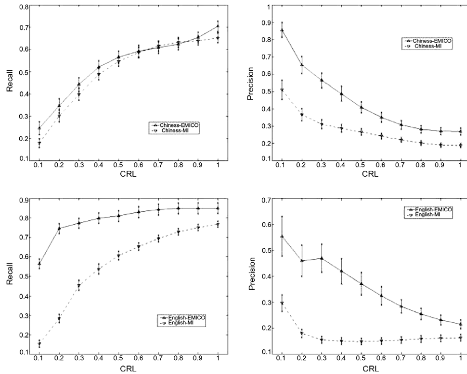
Fig. 6. The performances of mutual information and EMICO for Chinese and English substantival MWE extraction at different CRLs, respectively.
