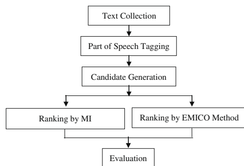
Fig. 5. The framework for comparison between MI and EMICO methods in substantial MWE extraction from Chinese and English text, respectively.
