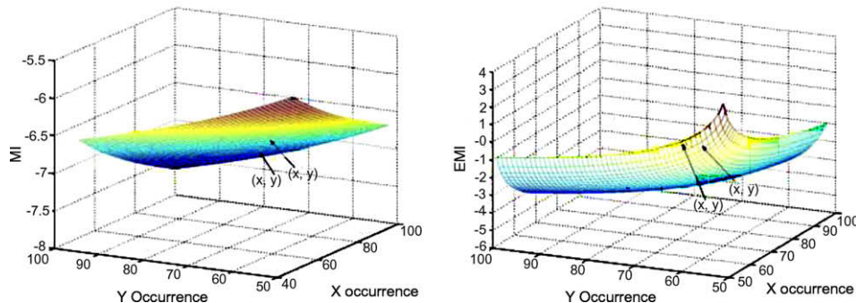
Fig. 3. Plots of MI (left) and EMI (right) for association measure of (x, y) and (x', y') , respectively. Their co-occurrence is fixed as 50 and occurrences of two words are varying in their axes.
